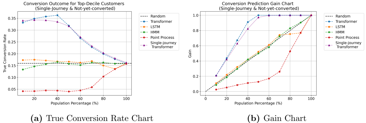
Figure 6: True Conversion Rate and Gain in Top Decile Single Journey and Not-yet-Converted Customers
