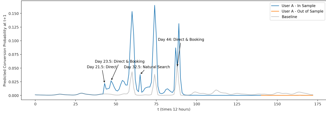
(a) User A - Booking Probability
