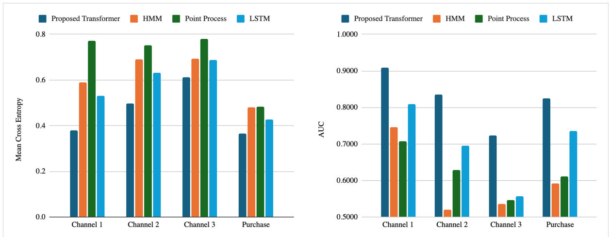
Figure 16: Model Comparisons under ARMA(2,2) DGP
