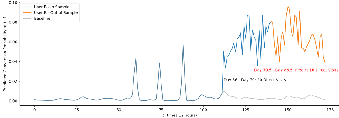
(b) User B - Booking Probability
