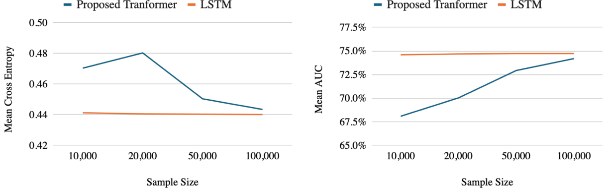
Figure 14: Transformer and LSTM Performance under Different Sample Size under AR5 DGP
