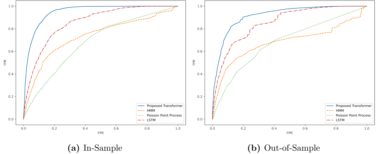
Figure 10: ROC curve of proposed model versus three benchmark models on the first 140 time periods.
