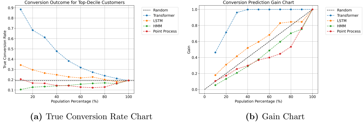
Figure 5: True Conversion Rate and Gain in Top Decile Customers
