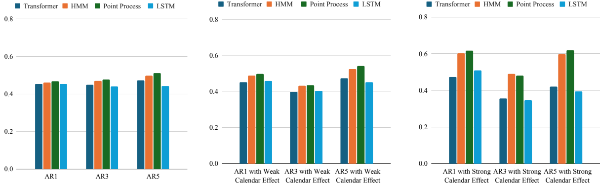
Figure 13: Mean Cross Entropy with True DGP Probability for AR Datasets
