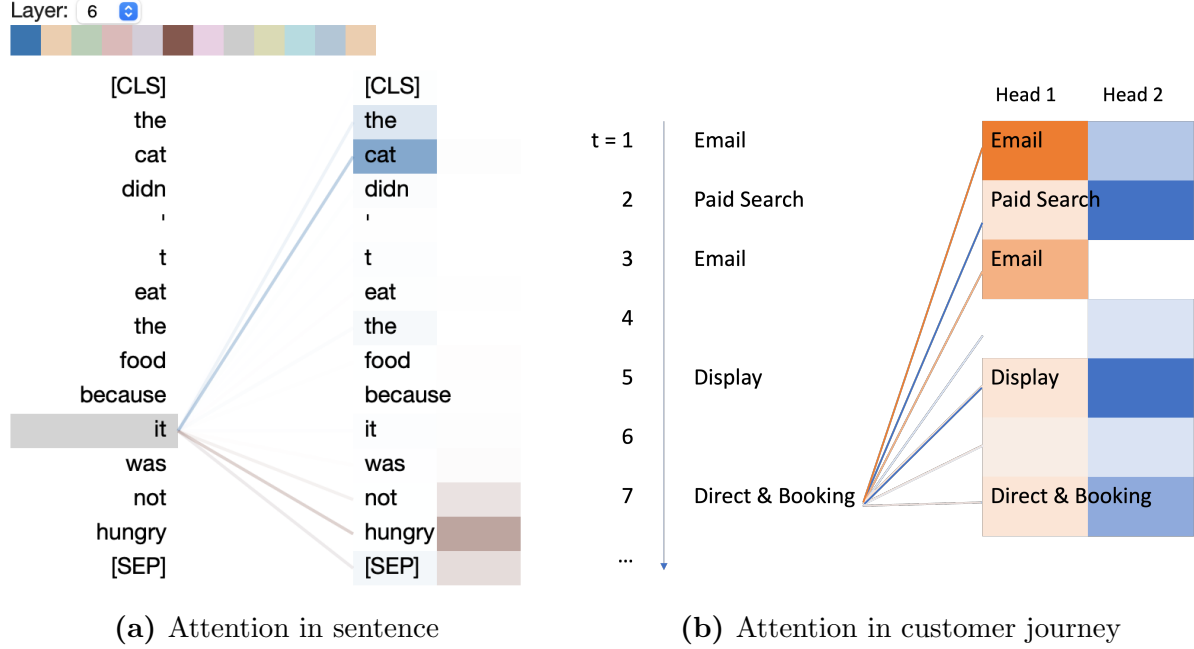
Figure 2: Illustrations of Multi-head Self-attention in Sentence and Customer Journey
