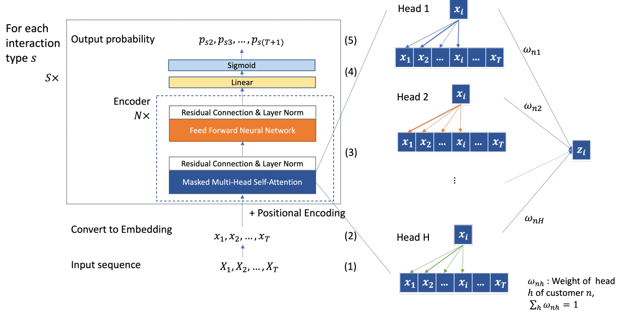
Figure 1: The architecture of the model
