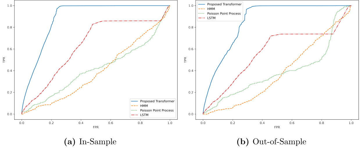
Figure 11: ROC curve of proposed model versus three benchmark models on the last 33 hold-out time periods.
