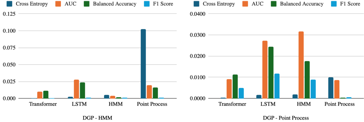
Figure 12: Mean Absolute Deviation from the Best Performing Model across the 50 Simulated Datasets
