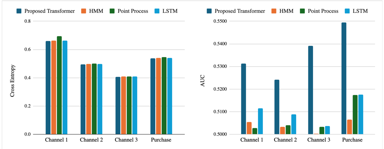
Figure 15: Model Comparisons under Mixture DGP
